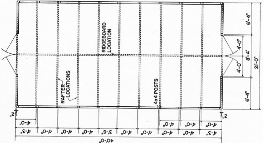
FLOOR PLAN SCALE: 1" = 4'
