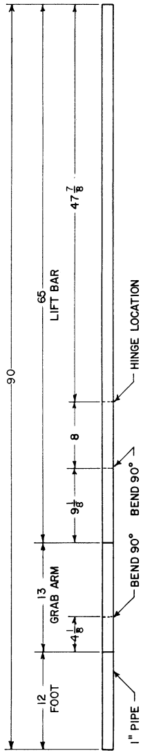
BLACK IRON PIPE CUTTING DIAGRAM SCALE: 3/8" = 1"
