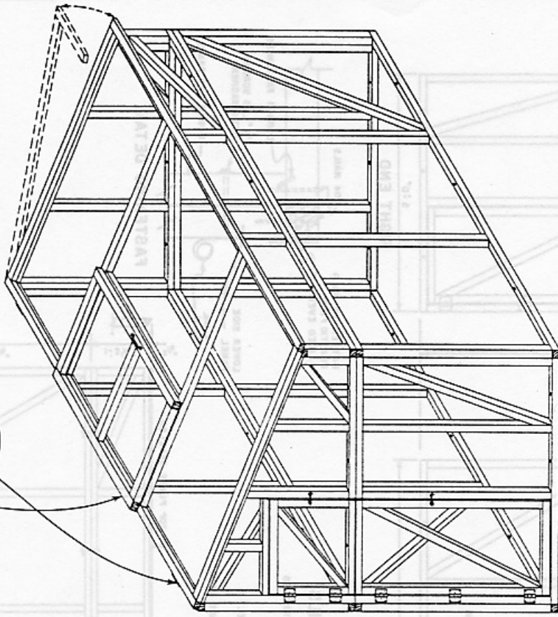
GREENHOUSE ASSEMBLY
